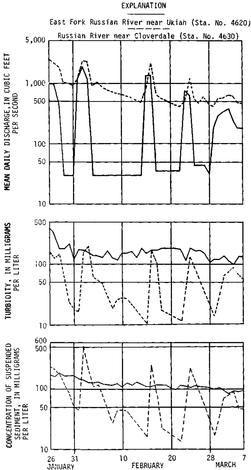
FIGURE 33.--Effect of releases from Lake Mendocino on the water discharge, turbidity, and concentration of suspended sediment at Russian River near Cloverdale, January-March 1965.
