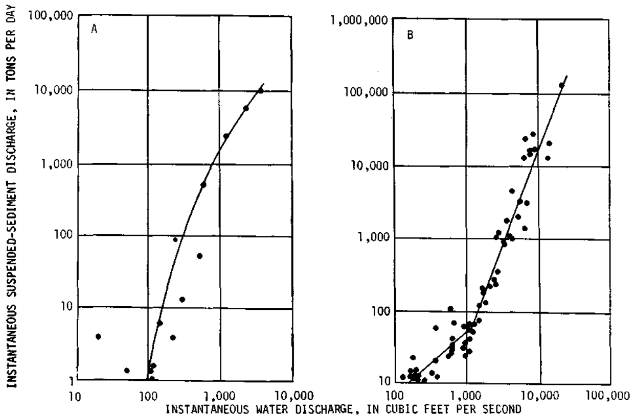
FIGURE 13.--Sediment-transport curves for A. Maacama Creek near Kellogg and B. Russian River near Guerneville.
