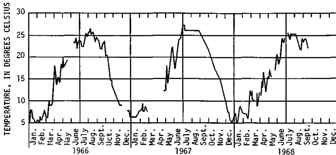
FIGURE 21.--Maximum daily temperatures of water near the surface of Lake Pillsbury, January 1966 to September 1968.
