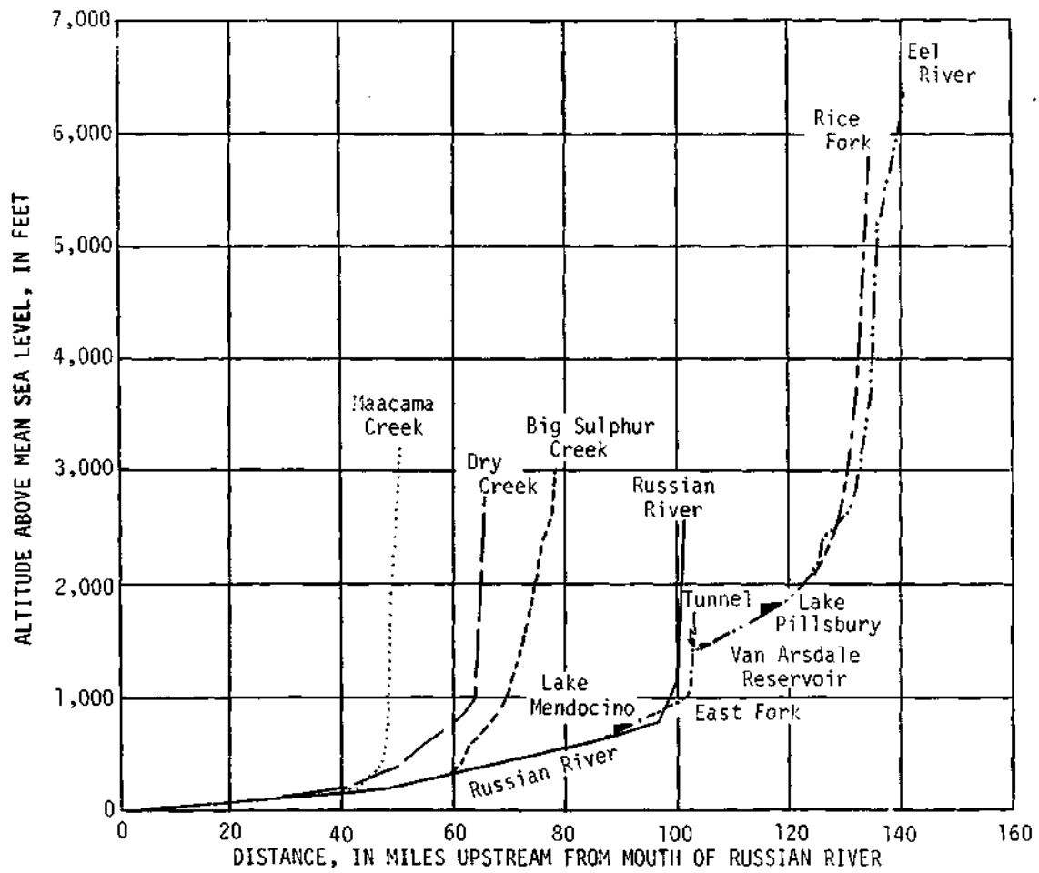
FIGURE 4.--Slopes of streams referred to in this report.
