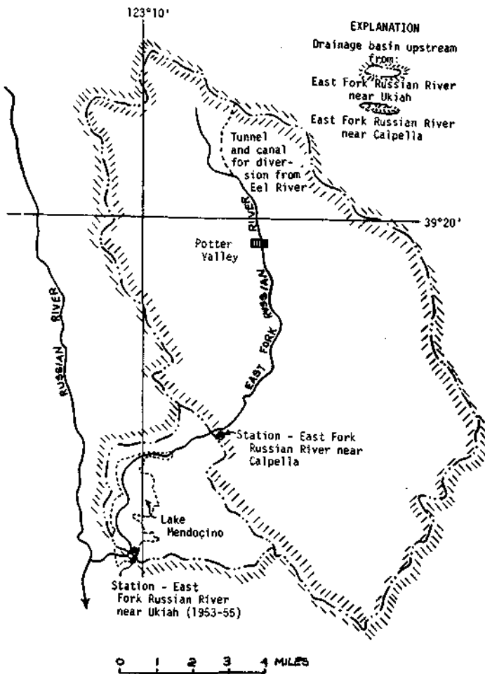
FIGURE 9.--Map of East Fork Russian River showing the stations on the East Fork Russian River near Calpella and near Ukiah (1953-55).
