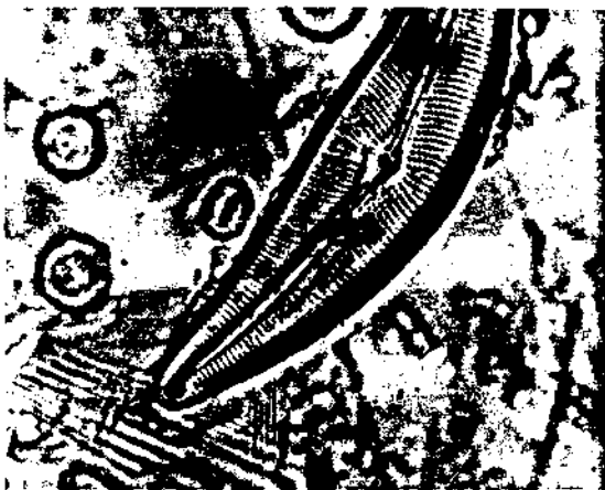
FIGURE 22.--Typical diatoms found in the suspended material in the Russian River basin. This sample was collected at the East Fork Russian River near Ukiah, June 24, 1964. Length of large diatom is about 0.11 mm.
