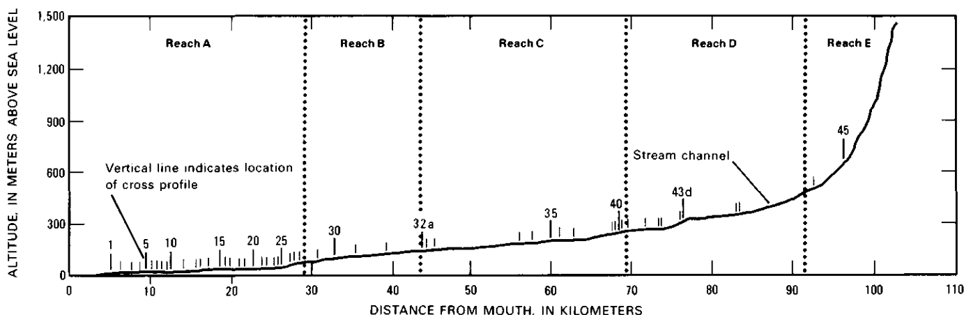
FIGURE 14.— Longitudinal profile of Redwood Creek showing location of study reaches and surveyed stream-channel cross profiles.
