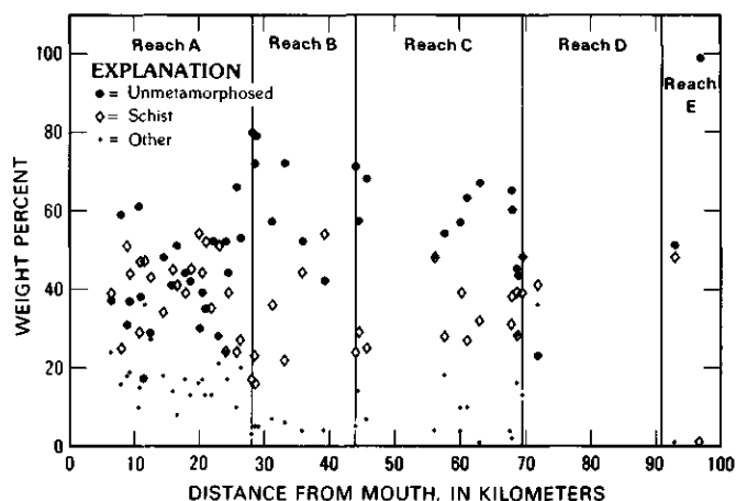
FIGURE 17. — Lithologic composition of bed material at cross profiles during the summer of 1976. "Unmetamorphosed" refers to conglomerate, sandstone, and mudstone clasts. "Schist" refers to schist and foliated metavolcanic clasts. "Other" refers to quartz and unfoliated greenstone clasts, and clasts too small for lithologic identification.
