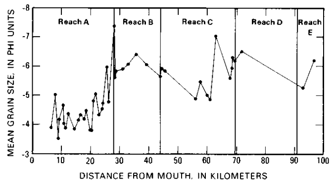
FIGURE 16.—Mean grain size of bed material at cross profiles during the summer of 1976.
