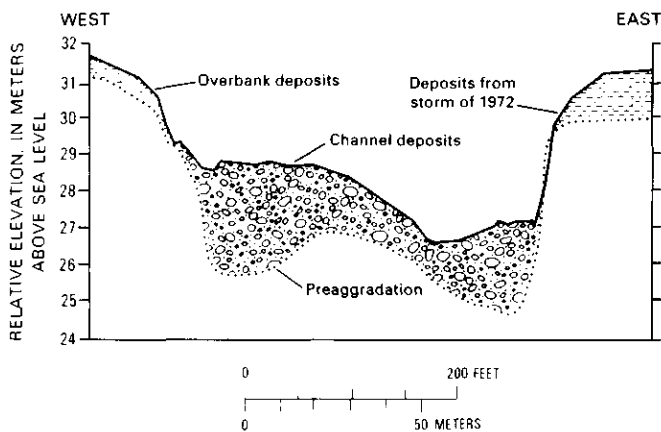
FIGURE 10. — Recent changes in the geometry of Redwood Creek at the mouth of Tom McDonald Creek. Preaggradation configuration was estimated from reports of local forest workers and road construction records. Configuration in 1972 is from ground surveys.
