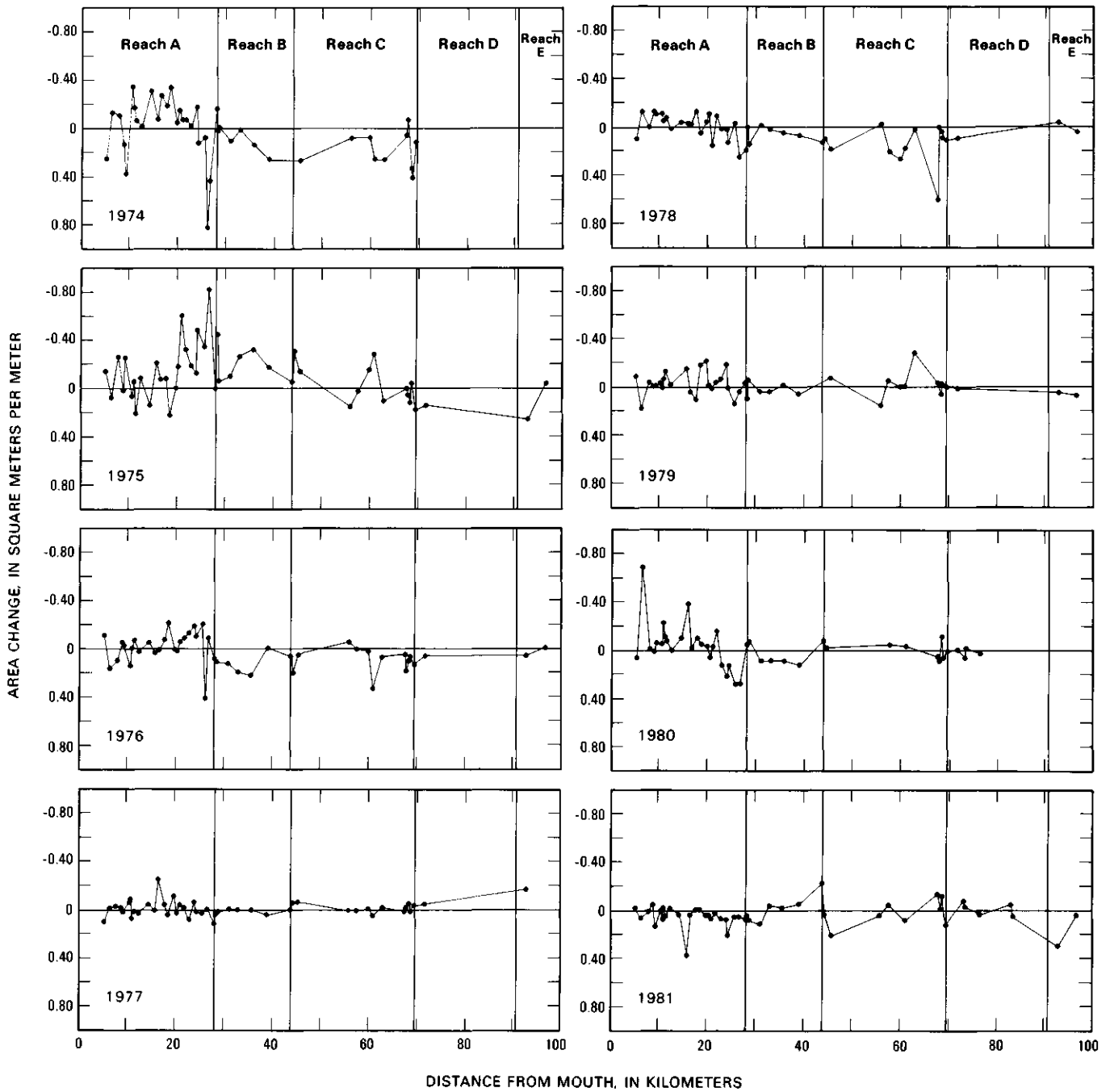
FIGURE 15. —Change in area of the streambed at cross profiles between water years 1974 and 1981. Area change is expressed in square meters of change per meter of bank-to-bank width. Channel scour is indicated by a positive change in area, and channel fill by a negative change. The lines connecting data points have no physical significance. They are presented only to aid in interpreting the data.
