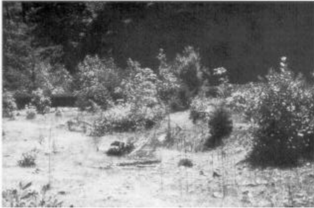
FIGURE 4. —Surface of gravel berm deposited (along a midbasin reach of Redwood Creek) during flood of December 1964. Photograph taken in August 1978. Alders in foreground are 1 to 1.5 m tall. Note small pack for scale.
