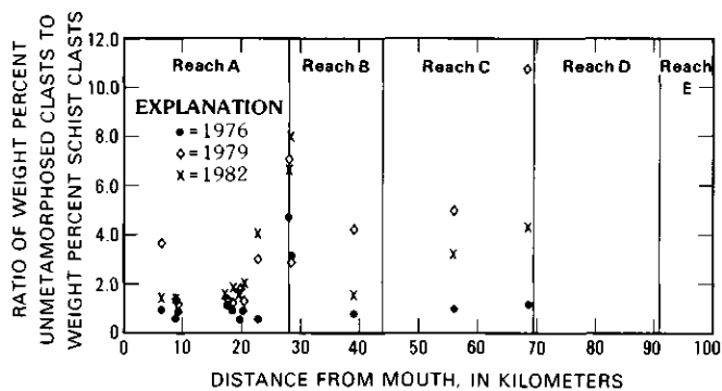
FIGURE 21.—Ratio of weight percent unmetamorphosed rocks to weight percent schist in bed material at selected cross profiles, summers of 1976 and 1982.
