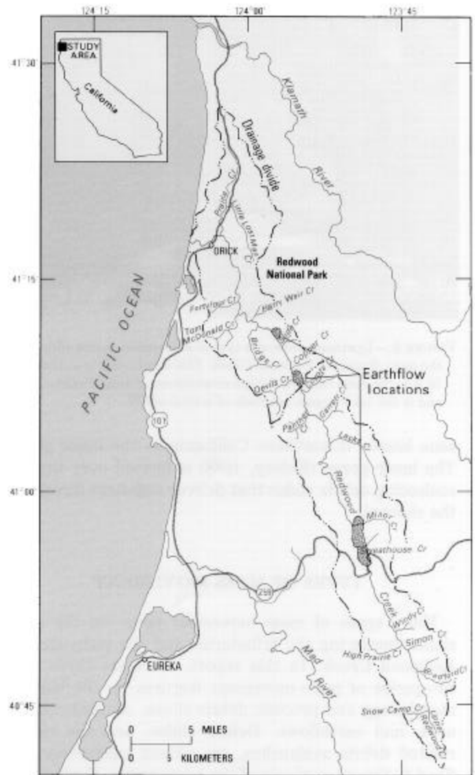
FIGURE 4. —Reaches where earthflows are abundant on the right bank of Redwood Creek (stippled areas). With one exception (the northernmost Counts Hill earthflow), the 16 earthflows occur along two distinct reaches of Redwood Creek.
