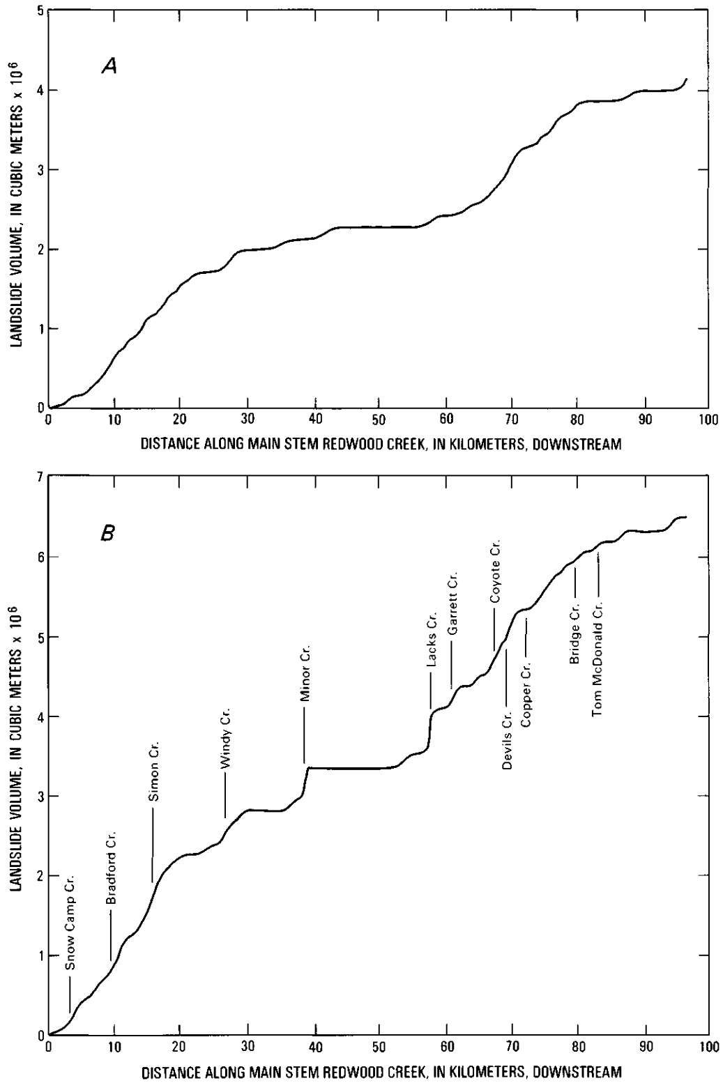
FIGURE 5.—Volume of sediment, cumulative through distance downstream along main-stem Redwood Creek, contributed by landslides for the period 1954-80. A , Volume contributed only by landslides along main stem, and B , Volume contributed by landslides along main stem and tributaries; location of tributary mouths is shown on graph. Note the two reaches of high input, kilometers 0 to 29 and kilometers 58 to 77.
