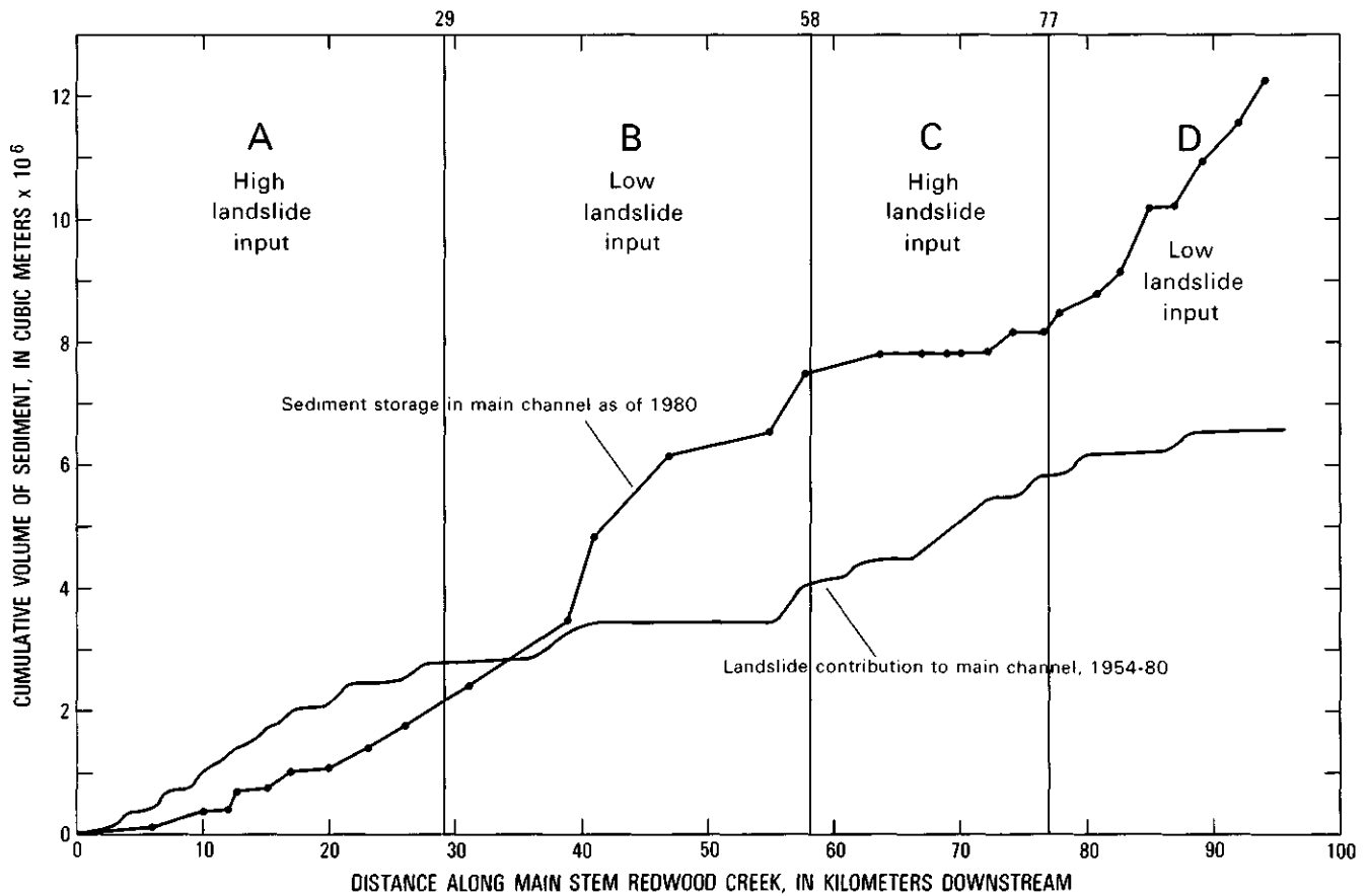
FIGURE 6.—Comparison of volume of sediment stored in main channel and volume of sediment contributed by landslides to main channel, both cumulative through distance downstream along the main channel of Redwood Creek. Reaches from kilometers 0 to 29
