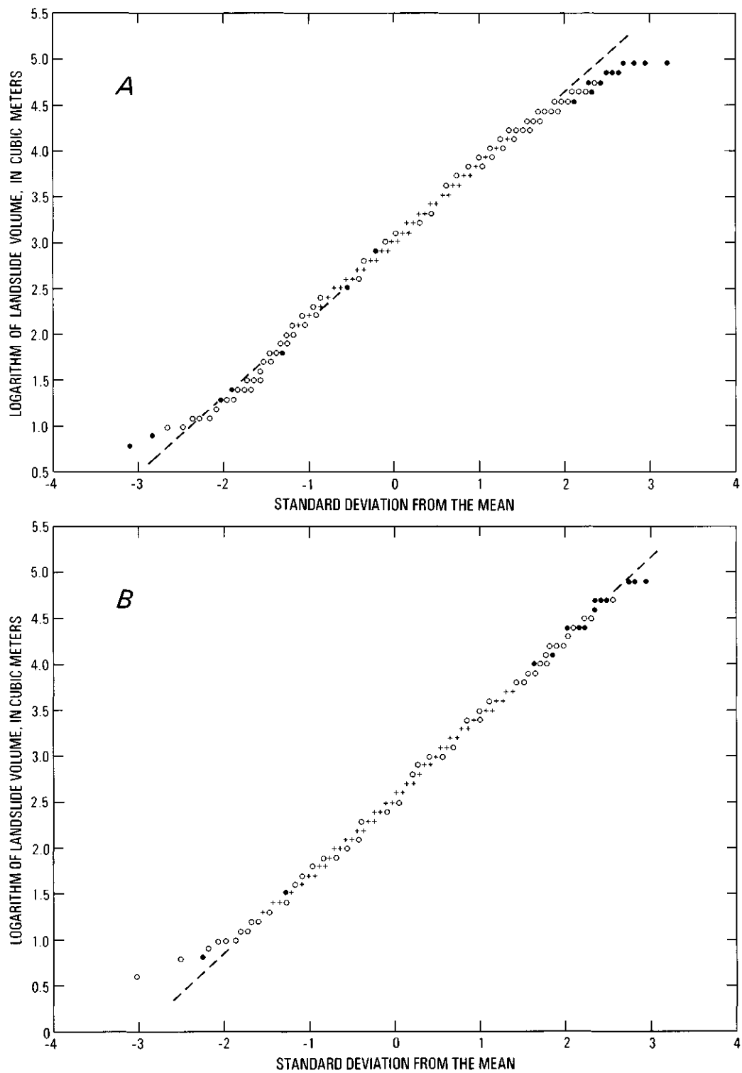
FIGURE 8. —Normal probability plot of the logarithm of landslide volume ( m^3 ). A, Landslides along the main stem of Redwood Creek, n=877 . B, Landslides along tributary channels, w=975 . Solid dots=1 landslide; open dots=2-9 landslides; crosses= \geq 10 landslides.
