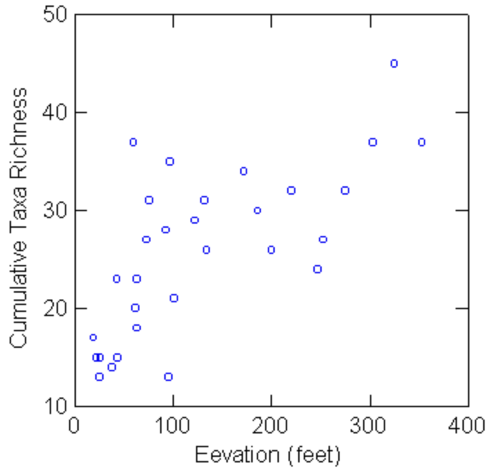
Figure 2. Relationship between cumulative Taxa Richness and elevation for all sites sampled in the four Marin County watersheds sampled during fall 1999 and spring 2000.
