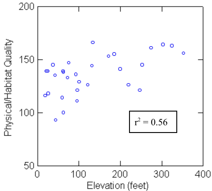
Figure 5. Relationship between cumulative Physical/Habitat Quality and elevation for all sites sampled in the four Marin County watersheds sampled during fall 1999 and spring 2000.
