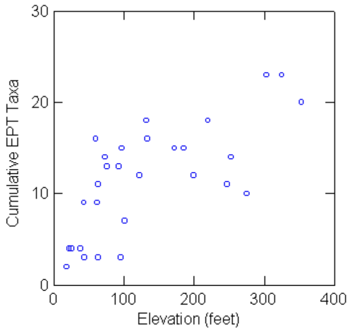
Figure 3. Relationship between cumulative EPT Taxa and elevation for all sites sampled in the four Marin County watersheds sampled during fall 1999 and spring 2000.
