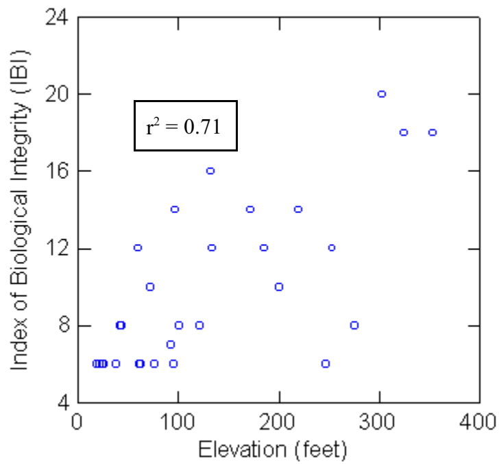
Figure 4. Relationship between Index of Biological Integrity (IBI) and elevation for all sites sampled in the four Marin County watersheds sampled during fall 1999 and spring 2000.
