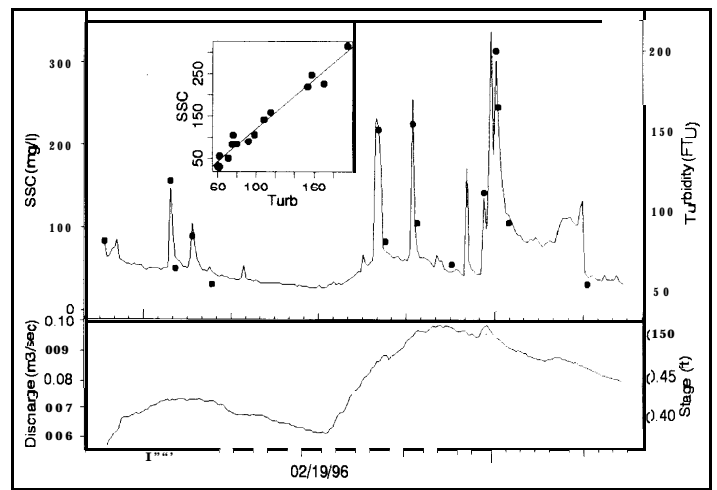
Figure 2. Turbidity, estimated and actual (sampled) suspended sediment concentration, and water discharge from a storm event in a 27-hectare tributary of Caspar Creek.
