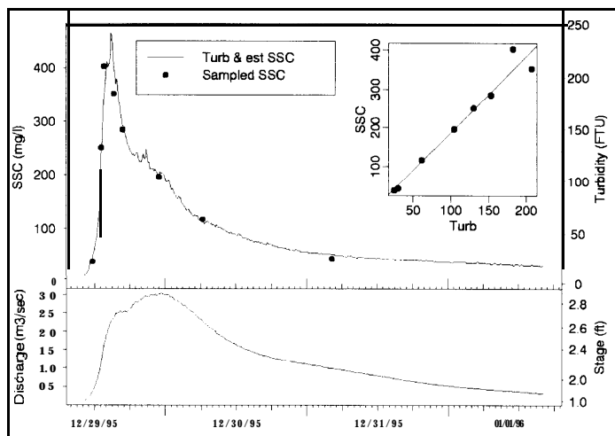
Figure 1. Turbidity, estimated and actual (sampled) suspended sediment concentration, and water discharge from a storm event at the 424-hectare Caspar Creek North Fork Weir.
