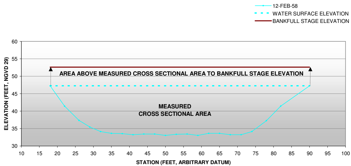
Figure 3. Method of Measuring the Channel Capacity
