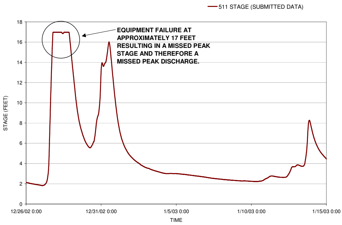
Figure 7. Hydrograph peaks at Station 511 illustrates why PALCO station 510 and 511 discharge data cannot be used for WY 2003
