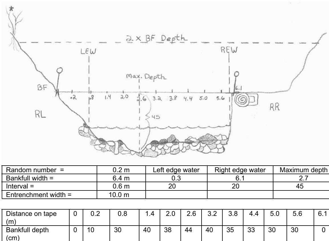
Figure II-3—Channel cross-section showing measurements.
