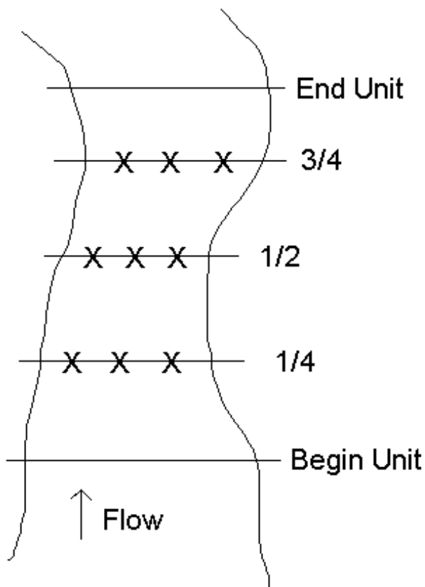
Figure 15. Location of bankfull width and depth measurements within habitat units. Bankfull and flood prone width measurements should be taken at \frac{1}{4} , \frac{1}{2} , and \frac{3}{4} of the length of the unit. Bankfull depth should be taken at \frac{1}{4} , \frac{1}{2} , and \frac{3}{4} of the bankfull width (indicated by X), with an additional depth location taken at the thalweg.
