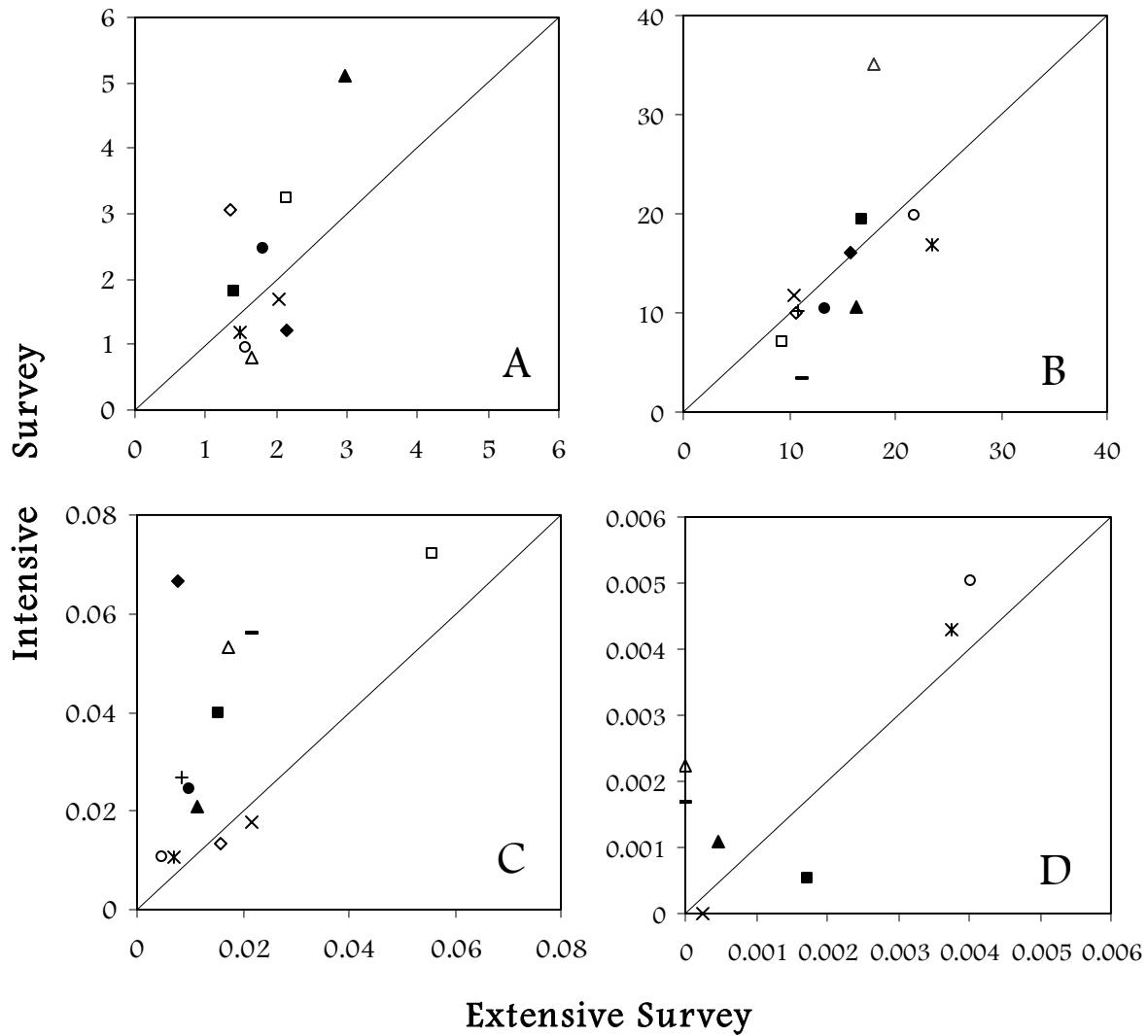
Figure 3. Comparison of extensive and intensive survey data. In all figures, data from the extensive survey are shown on the x-axis and data from the intensive survey are shown on the y-axis. Entrenchment ratio is shown in panel A, bankfull width: depth in panel B, total pool frequency in panel C (# / m), and frequency of pools greater than 1 m deep (# / m) in panel D. Symbols on the figures represent different watersheds, and individual watersheds are represented by the same symbol on all panels. Diagonal lines represent the one to one ratio.
