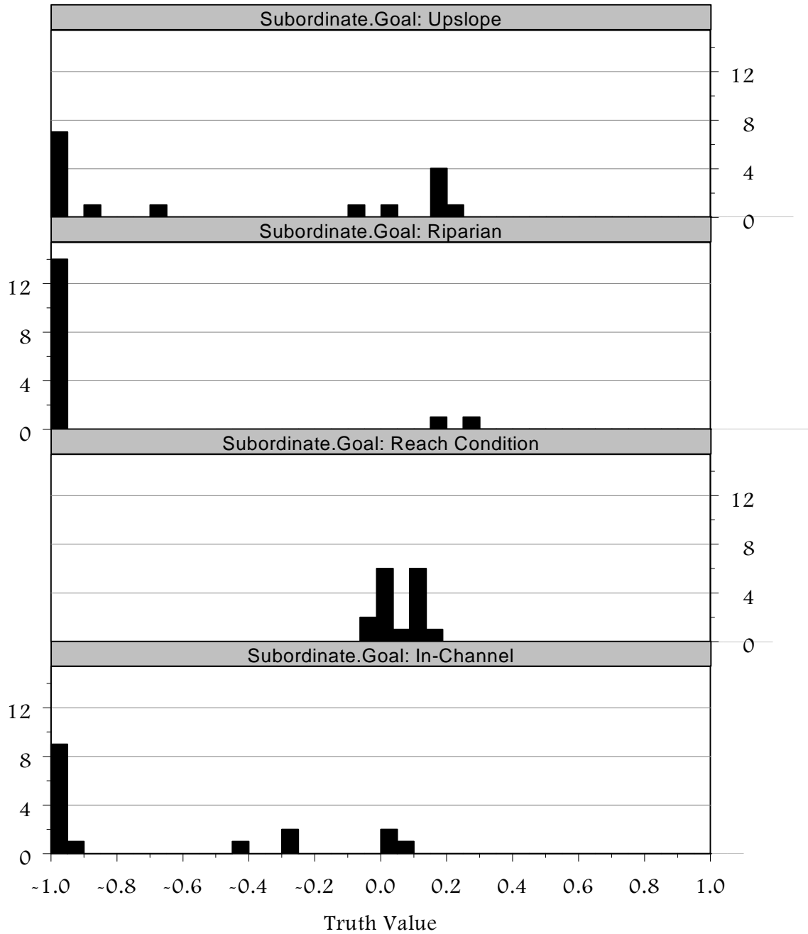
Figure 12. Frequency distribution of the truth values from four subordinate goals for watershed health. Note that -1.0 represents a false value for the goal, 0.0 represents either no data or an evaluation of zero, and 1.0 represents a true value for the goal. Labels correspond to the panel below. Each vertical bar represents a surveyed watershed.
