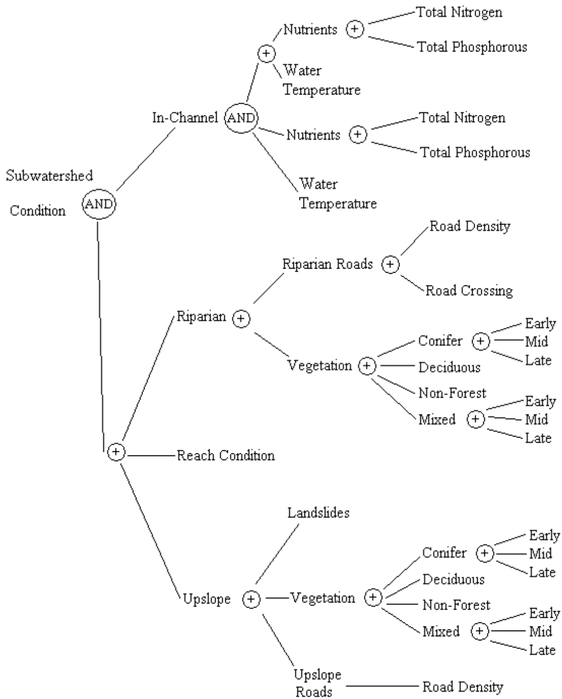
Figure 8. Watershed-level knowledge base used in the decision support model. The AND operators pass the lowest evaluation score, and + operators pass the average evaluation score to the next highest level.
