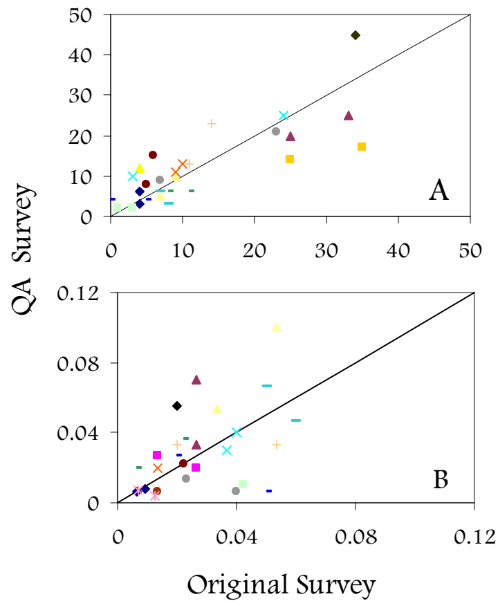
Figure 5. Comparison of original and QA surveys for habitat indicators. Wood frequency is shown in panel A in pieces per 100m, and pool frequency is shown in panel B in number of pools per meter. Points represent individual sample sites. Symbols on the figures represent different watersheds, and individual watersheds are represented by the same symbol on both panels. Diagonal lines represent the one to one ratio.
