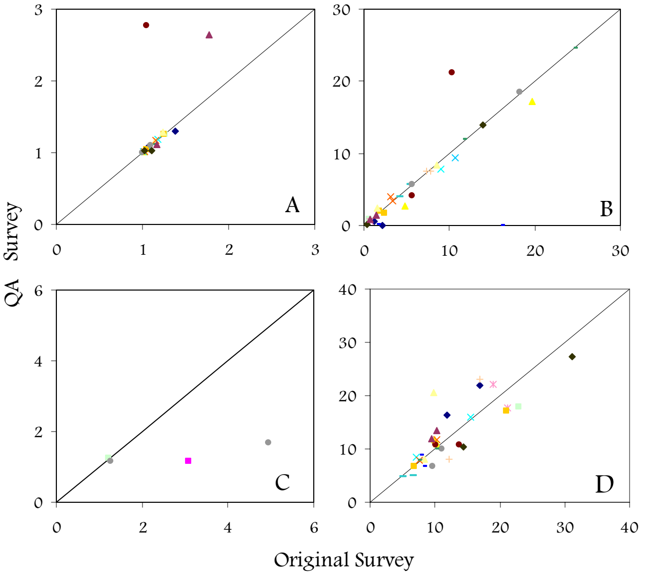
Figure 4. Comparison of original and QA surveys for channel morphology indicators. Sinuosity is shown in panel A, percent slope is shown in panel B, entrenchment ratio is shown in panel C, and bankfull width: depth is shown in panel D. Points represent individual sample sites. Symbols on the figures represent different watersheds, and individual watersheds are represented by the same symbol on all panels. Diagonal lines represent the one to one ratio.
