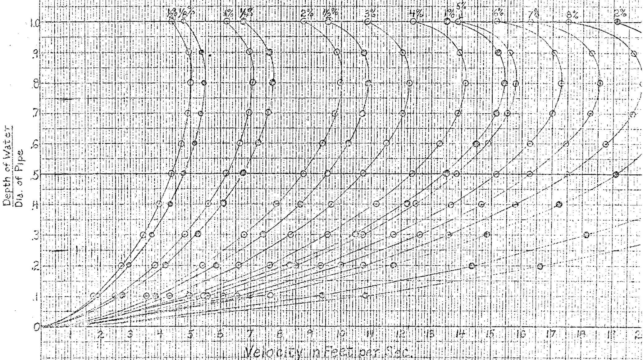
48" \phi Culverts
